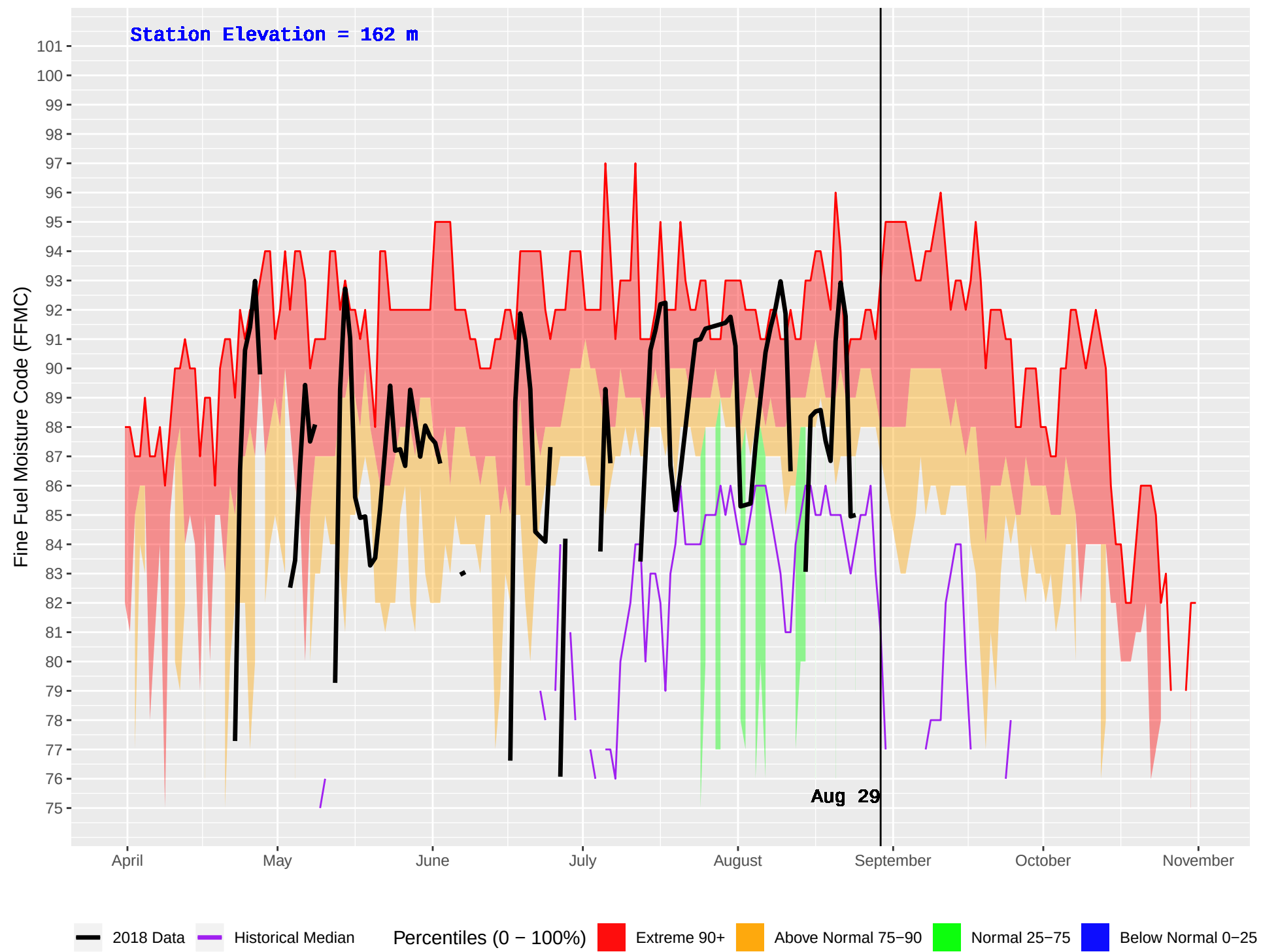
UBC RESEARCH (72) : Historical (1981–2016) and Current (2018) Daily Fine Fuel Moisture Code (FFMC)
