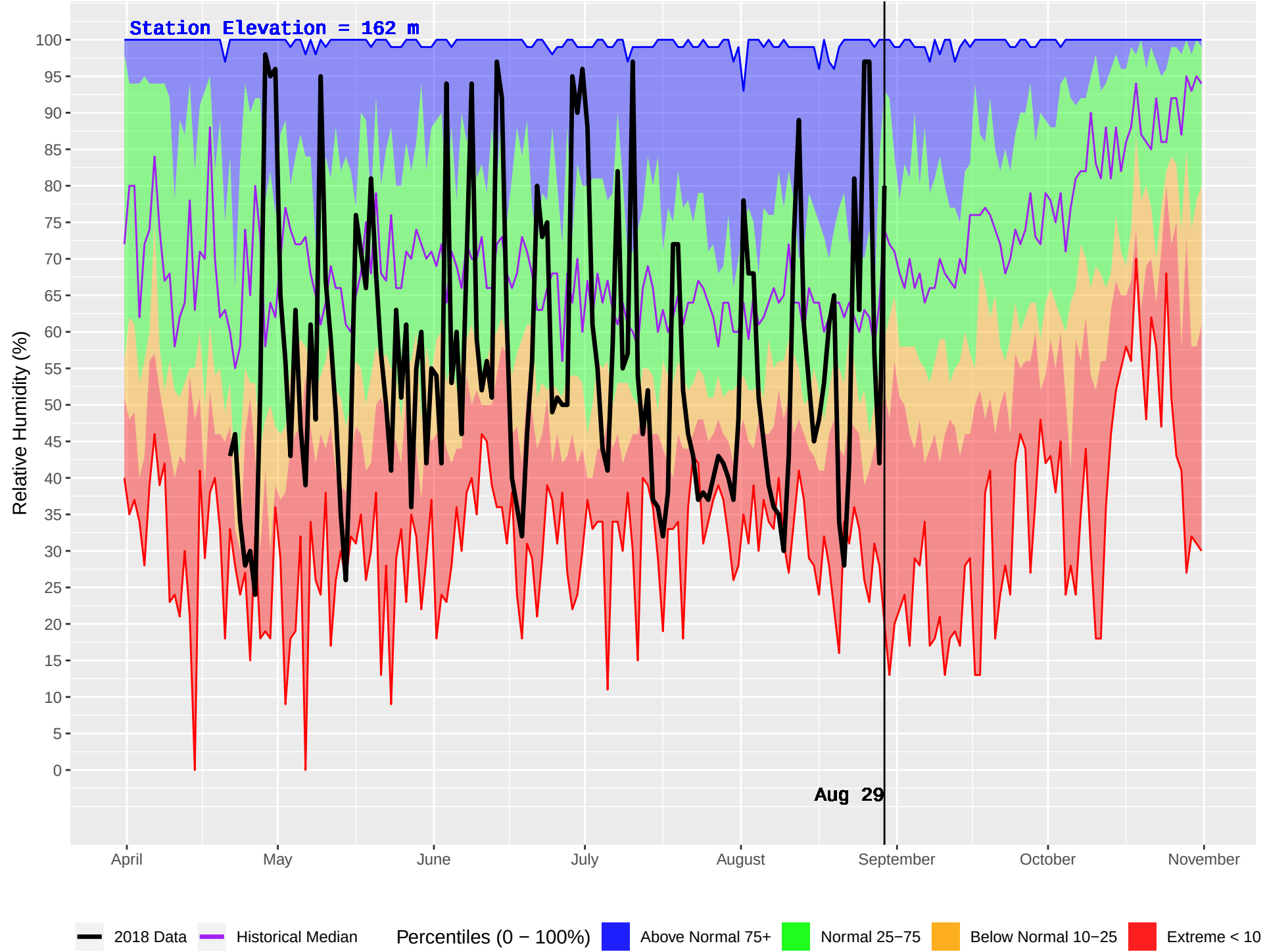
UBC RESEARCH (72) : Historical (1981–2016) and Current (2018) Daily Relative Humidity
