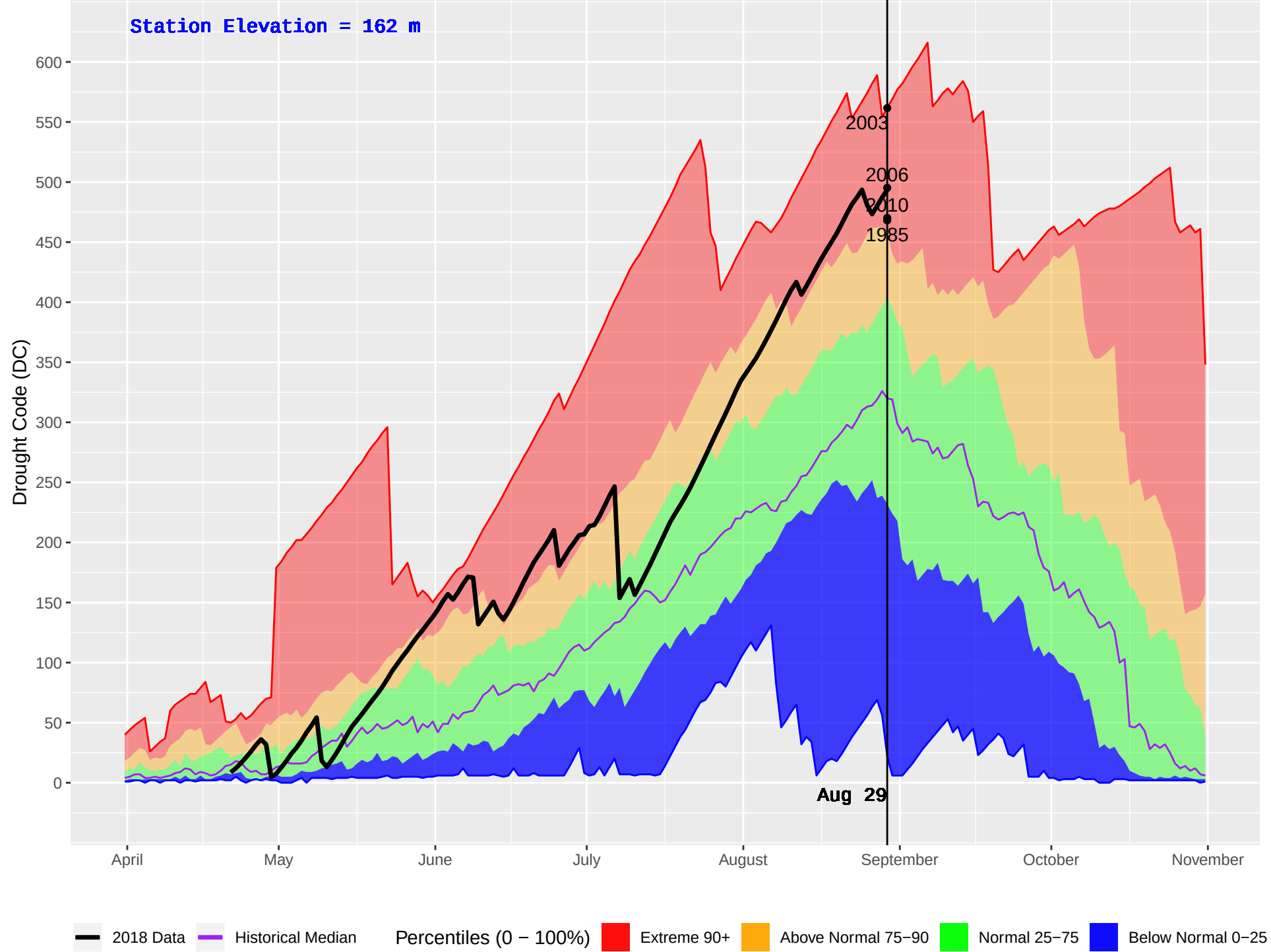
UBC RESEARCH (72) : Historical (1981–2016) and Current (2018) Daily Drought Code (DC)
