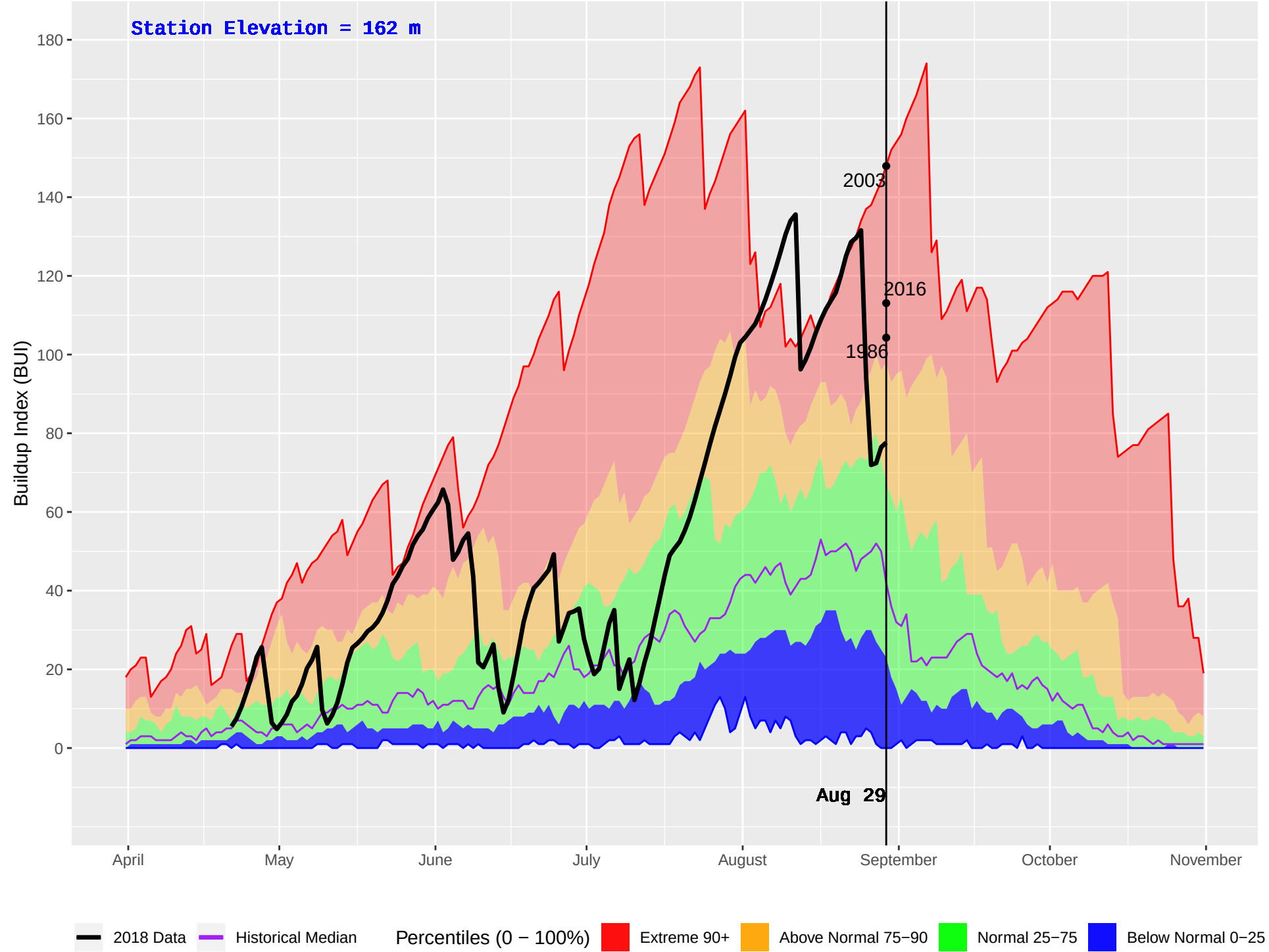
UBC RESEARCH (72) : Historical (1981–2016) and Current (2018) Daily Buildup Index (BUI)
